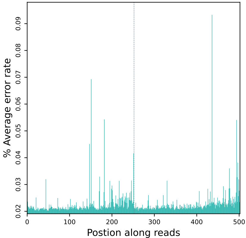
Error rate distribution along reads (R10501)
